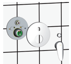
Slide the plate support over the cartridge and the diverter and screw into the right position. Then mount the visible design parts.
