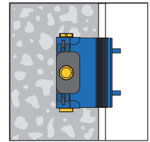
In-wall installation.
