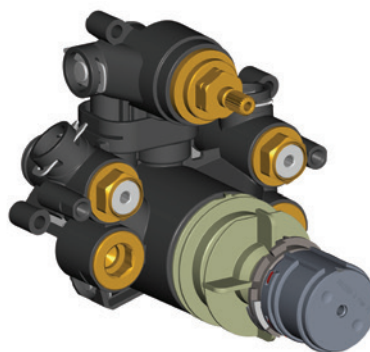
Thermostat Long-lasting thermostatic cartridge, side valves for pre-shut off with non return valve and DICHT-FIX.
