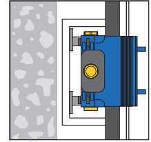
Installation on pre-carrier systems.
