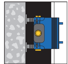
In-front-of-wall installation.
