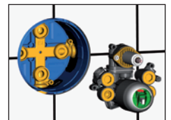
Assemble the function unit (thermostat or single lever body) from Kit 2 and verify watertightness.
