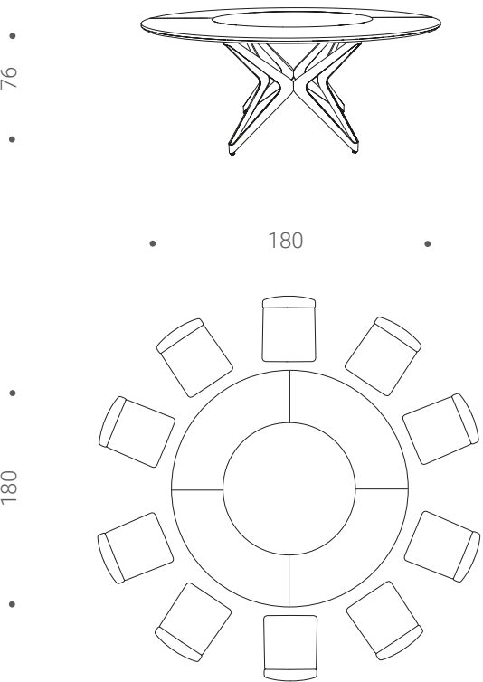
Tavolo T254 DNA piano PZ51 vassoio centrale CC10 struttura MT98 / Poltroncina S456 THELMA seduta P11 base PZ51 - Table T254 DNA top PZ51 central tray CC10 structure MT98 / Armchair S456 THELMA covering P11 structure PZ51 - Tisch T254 DNA platte PZ51 zentrales Fach CC10 Untergestell MT98 / Sessel S456 THELMA Besichtigung P11 Struktur PZ51 - Table T254 DNA plateau PZ51 plateau central CC10 structure MT98 / Fauteuil S456 THELMA Revêtement P11 structure PZ51 - Mesa T254 DNA sobre PZ51 bandeja central CC10 estructura MT98 / Sillón S456 THELMA tapizado P11 estructura PZ51 - Стол T254 DNA Топ PZ51 центральный лоток CC10 Структура MT98 / Кресло S456 THELMA Обивка P11 Структура PZ51
